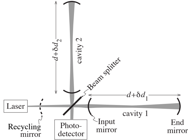
Fig. 9.11: Laser Interferometer Gravitational Wave Detector.
