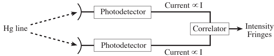
Fig. 9.12: Hanbury-Brown and Twiss Intensity Interferometer.
