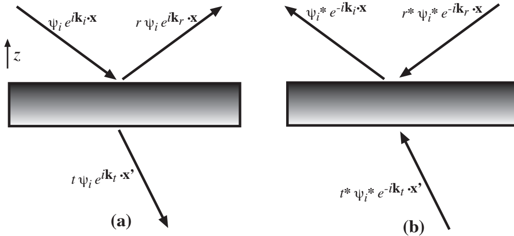
Fig. 9.9: Construction for deriving reciprocity relations for amplitude transmission and reflection coefficients.
