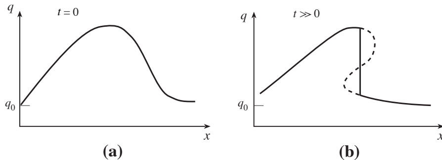
Fig. 17.8: Evolution of a nonlinear sound wave. The fluid at the crest of the wave moves faster than the fluid in the trough. Mathematically, the flow eventually becomes triple-valued. Physically, a shock wave develops.
