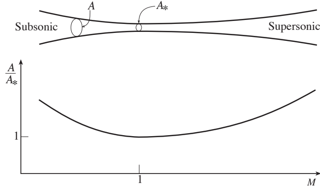
Fig. 17.4: Variation of cross sectional area, A , of a narrow bundle of flow lines as the Mach number, M , increases. Note that the flow is transonic ( M = 1 ) when A is at its minimum, A_* .
