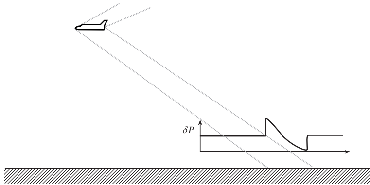
Fig. 17.13: Double shock created by supersonic projectile and associated “N wave” pressure distribution.
