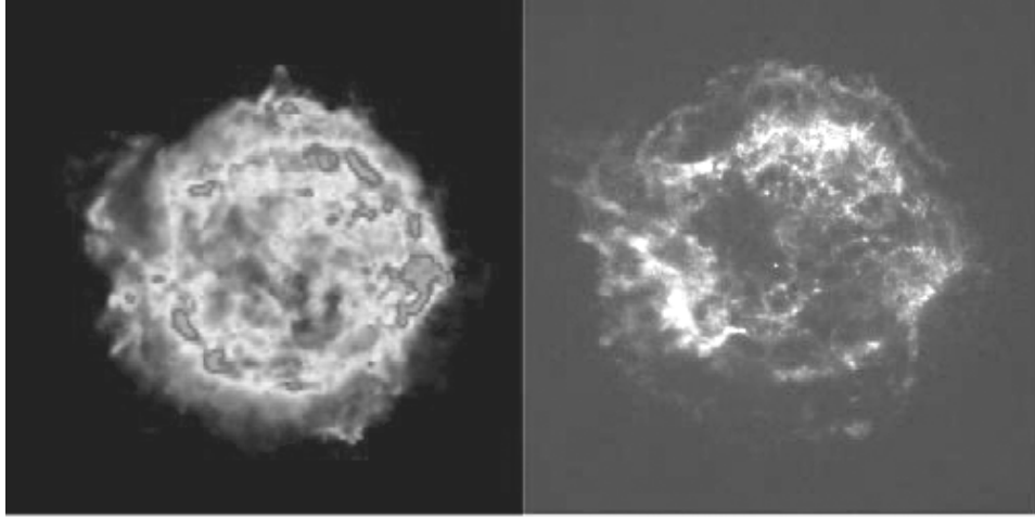
Fig. 17.18: Cassiopeia A – a supernova remnant left behind an exploding star in our galaxy approximately 300 years ago. The image to the left is made using the Very Large Array Radio Telescope; that to the right by the Chandra X-ray Observatory.
