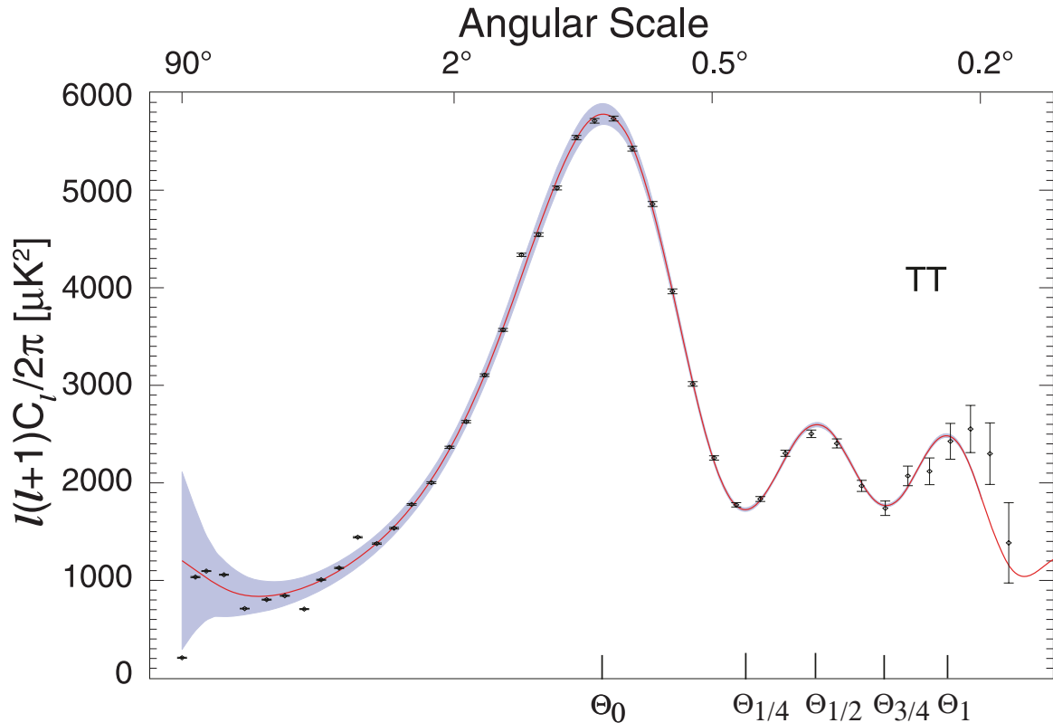
Fig. 27.6: Anisotropy of the CMB as measured by WMAP (the first two Doppler peaks; most error bars smaller than the dots; Hinshaw et. al. 2009) and by CBI and ACBAR (the last three peaks; Pearson et. al. 2002, and Kuo et. al. 2002). Plotted vertically is the mean square temperature fluctuation; plotted horizontally is the angular scale \Theta . The solid curve is the theoretical prediction when one inserts the best-fit values of the cosmological parameters. The grey shading is the range of statistical fluctuations one would expect in an ensemble of universes all with these same cosmological parameter values. This figure is adapted from Hinshaw et. al. (2009).
