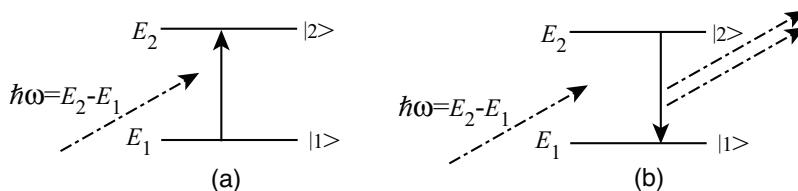
Fig. 10.1: (a) Photon Absorption : A photon with energy \hbar\omega = E_2 - E_1 excites a molecule from its ground state, with energy E_1 to an excited state with energy E_2 (as depicted by an energy-level diagram). (b) Stimulated Emission : The molecule is initially in its excited state, and the incoming photon stimulates it to deexcite into its ground state, emitting a photon identical to the incoming one.
