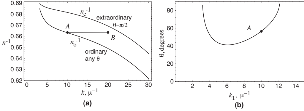
Fig. 10.10: (a) The inverse of the index of refraction \mathbf{n}^{-1} (equal to the phase speed in units of the speed of light) for electromagnetic waves propagating at an angle \theta to the symmetry axis of a KDP crystal, as a function of wave number k in reciprocal microns. See Eq. (10.36a) for lower curve and Eq. (10.36b) with \theta = \pi/2 for upper curve. For extraordinary waves propagating at an arbitrary angle \theta to the crystal's symmetry axis, \mathbf{n}^{-1} is a mean [Eq. (10.36b)] of the two plotted curves. (b) The angle \theta to the symmetry axis at which ordinary waves with wave number k_1 (e.g. point A ) must propagate in order that 3-wave mixing be able to produce frequency doubled or phase conjugated extraordinary waves (e.g. point B ).
