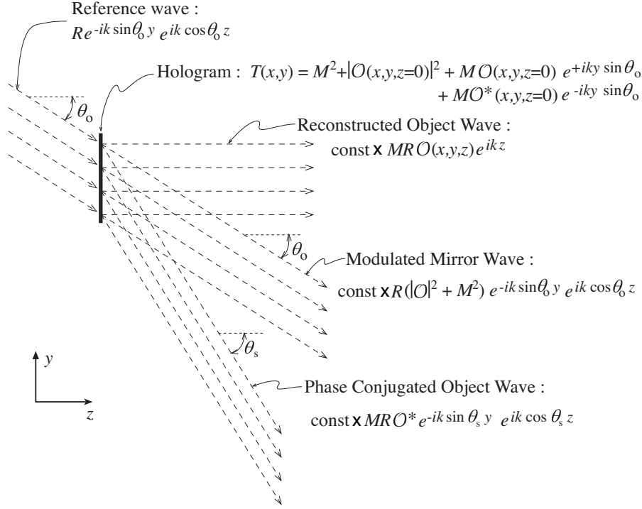
Fig. 10.7: Reconstructing the holographic image from the hologram. Note that \sin \theta_s = 2 \sin \theta_o .
