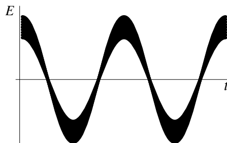
Fig. 10.12: The error band for the electric field E(t) , as measured at a fixed location in space when squeezed light with reduced phase noise passes by.
