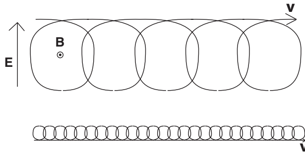
Fig. 19.4: The proton motion (upper diagram) and electron motion (lower diagram) orthogonal to the magnetic field, when there are constant electric and magnetic fields with |\mathbf{E} \times \mathbf{B}| < B^2c . Each electron and proton moves in a circle with a superposed drift velocity \mathbf{v}_D given by Eq. (19.56).
