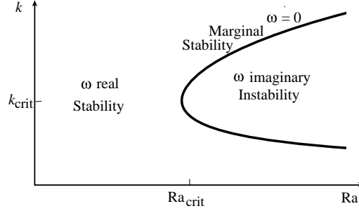
Fig. 18.2: Horizontal wave number k of the first mode to go unstable, as a function of Rayleigh number, Ra . Along the solid curve the mode has zero frequency; to the left of the curve it is stable, to the right it is unstable. Ra_{\text{crit}} is the minimum Rayleigh number for convective instability.
