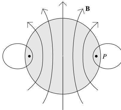
Fig. 19.11: Impossibility of an axisymmetric dynamo.
