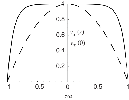
Fig. 19.9: Velocity profiles [Eq. 19.39] for flow in an electromagnetic pump of width 2a with small and large Hartmann number scaled to the velocity at the center of the channel. Dashed curve: the almost parabolic profile for H = 0.1 [Eq. (19.35)]. Solid curve: the almost flat topped profile for H = 10 .
