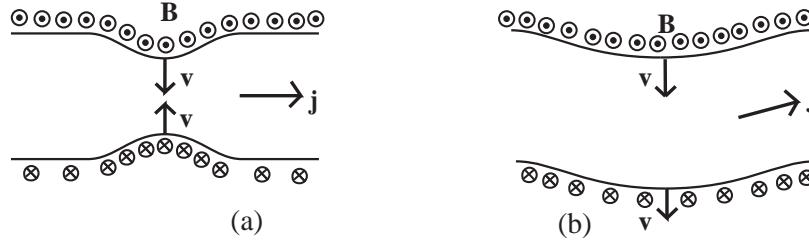
Fig. 19.10: Physical interpretation of a) sausage and b) kink instabilities.
