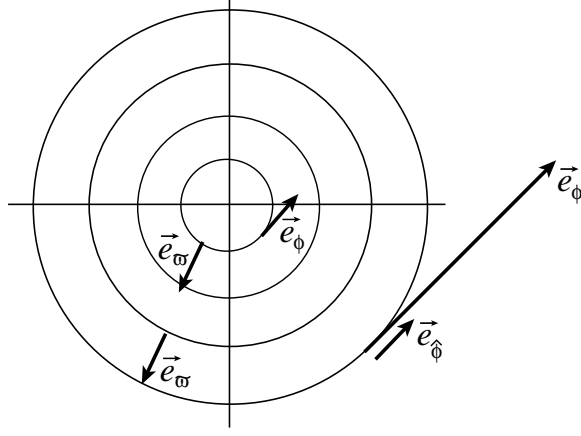
Fig. 24.3: A circular coordinate system \{\varpi, \phi\} and its coordinate basis vectors \vec{e}_\varpi = \partial\mathcal{P}/\partial\varpi , \vec{e}_\phi = \partial\mathcal{P}/\partial\phi at several locations in the coordinate system. Also shown is the orthonormal basis vector \vec{e}_{\hat{\phi}} .
