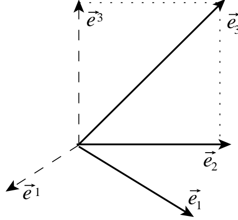
Fig. 24.2: Non-orthonormal basis vectors \vec{e}_j in Euclidean 3-space and two members \vec{e}^1 and \vec{e}^3 of the dual basis. The vectors \vec{e}_1 and \vec{e}_2 lie in the horizontal plane, so \vec{e}^3 is orthogonal to that plane, i.e. it points vertically upward, and its inner product with \vec{e}_3 is unity. Similarly, the vectors \vec{e}_2 and \vec{e}_3 span a vertical plane, so \vec{e}^1 is orthogonal to that plane, i.e. it points horizontally, and its inner product with \vec{e}_1 is unity.
