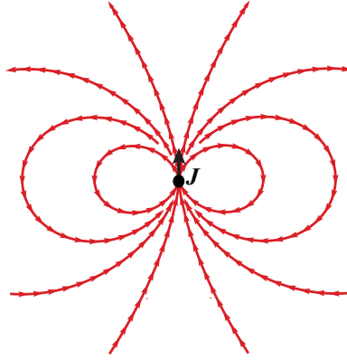
Fig. 25.5: The precessional angular velocity \Omega_{\text{fd}} [Eq. (25.100)] of an inertial-guidance gyroscope at rest outside a stationary, linearized source of gravity that has angular momentum \mathbf{J} . The arrows are all drawn with the same length rather than proportional to the magnitude of \Omega_{\text{fd}} .
