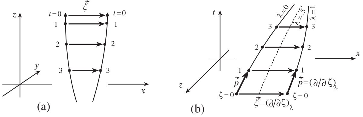
Fig. 25.3: The effects of tidal gravity on the relative motions of two freely falling particles. Diagram (a) depicts this in a Euclidean 3-space diagram using Newton’s theory of gravity. Diagram (b) depicts it in a spacetime diagram using Einstein’s theory of gravity, general relativity.
