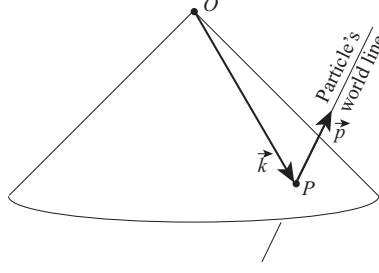
Fig. 25.4: The past light cone of an observation event \mathcal{O} , the world line of a particle, and two 4-vectors: the particle's 4-momentum \vec{p} at the point \mathcal{P} where it passes through \mathcal{O} 's past light cone, and the past-directed null vector \vec{k} that reaches from \mathcal{O} to \mathcal{P} .
